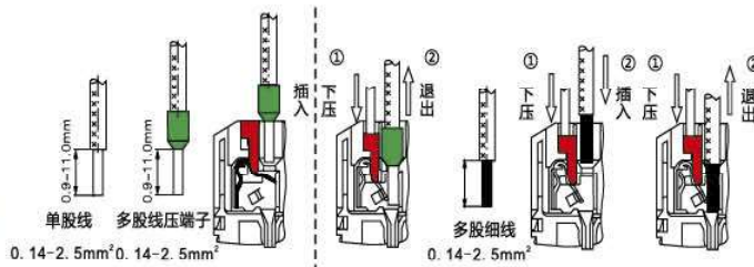
Step 2:接线完成 Connection completion
